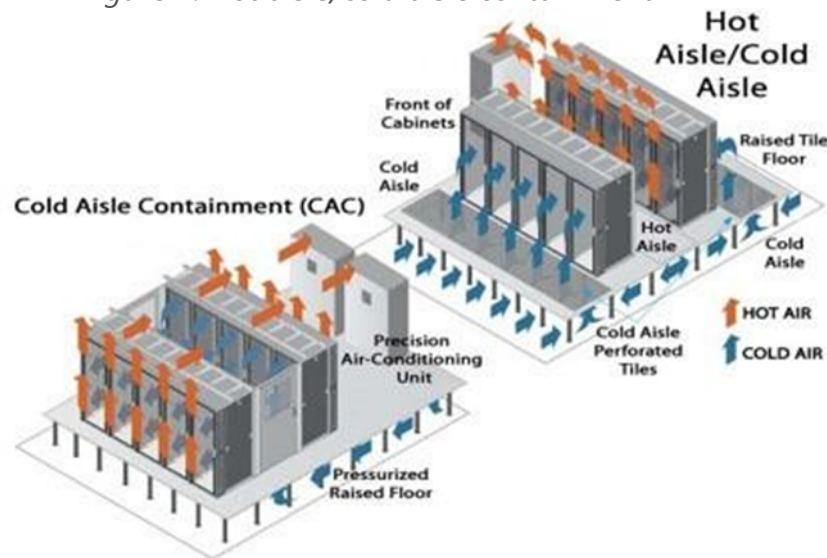
Figure 7: Hot aisle/cold aisle containment
