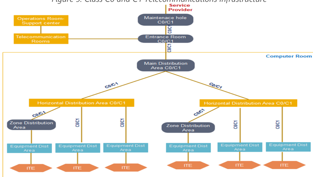
Figure 9: Class C0 and C1 Telecommunications Infrastructure
