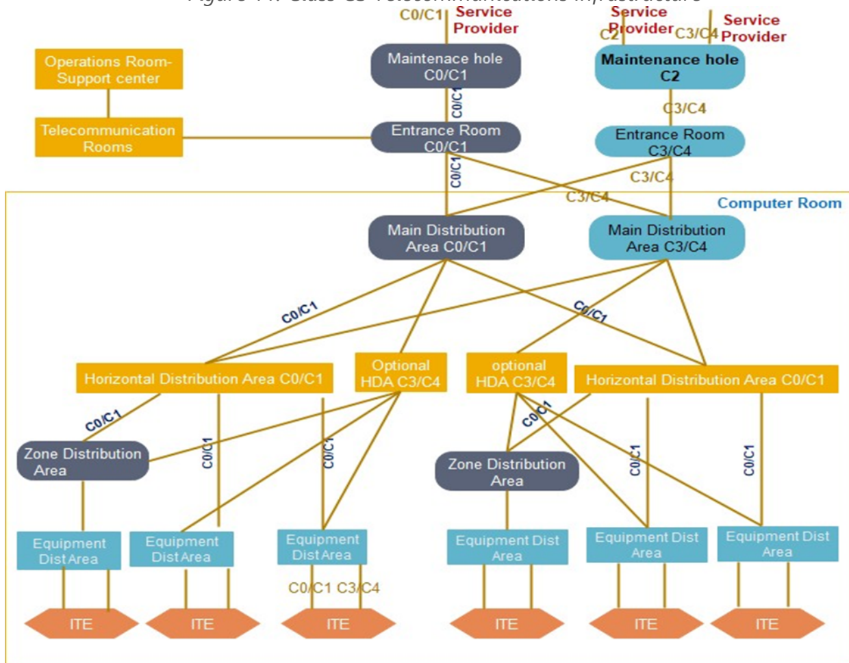
Figure 11: Class C3 Telecommunications Infrastructure
