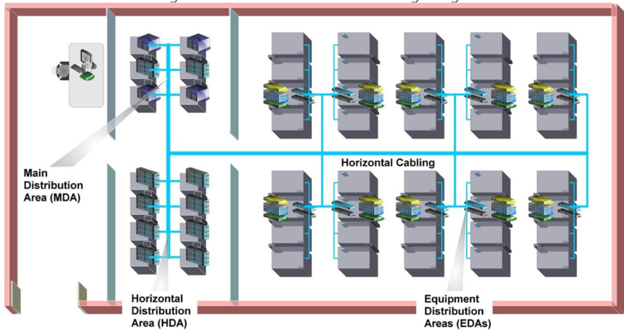
Figure 8: Data Centre network cabling design
