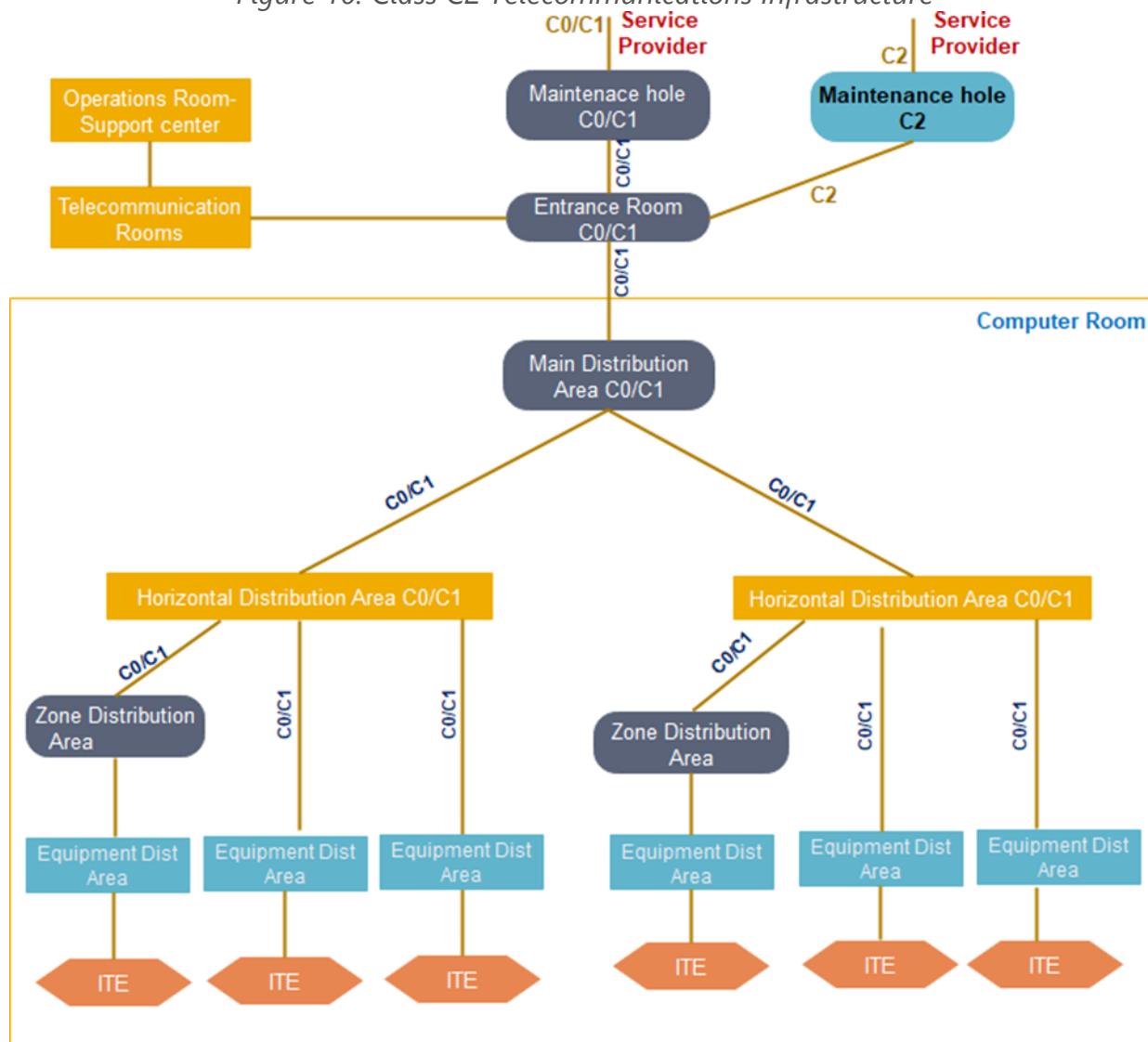
Figure 10: Class C2 Telecommunications Infrastructure
