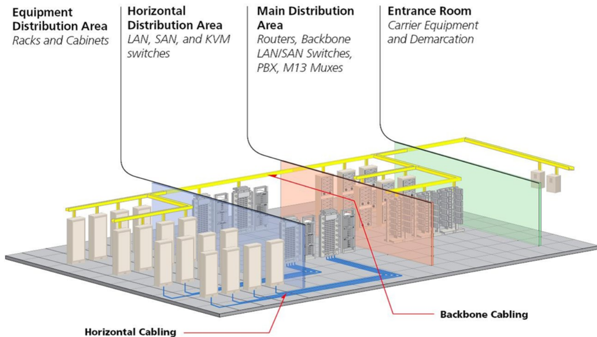
Figure 12: Cabling Topology
